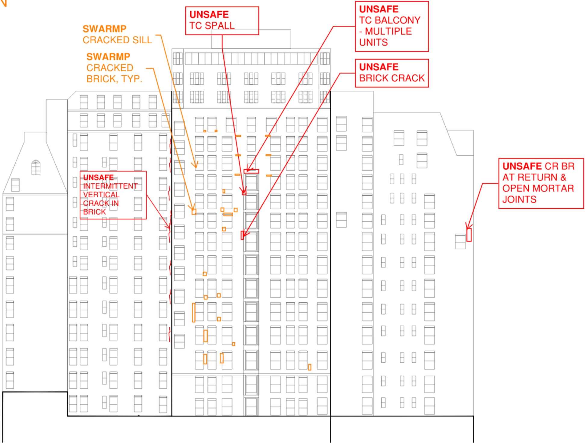
WEST COURTYARD ELEVATION
