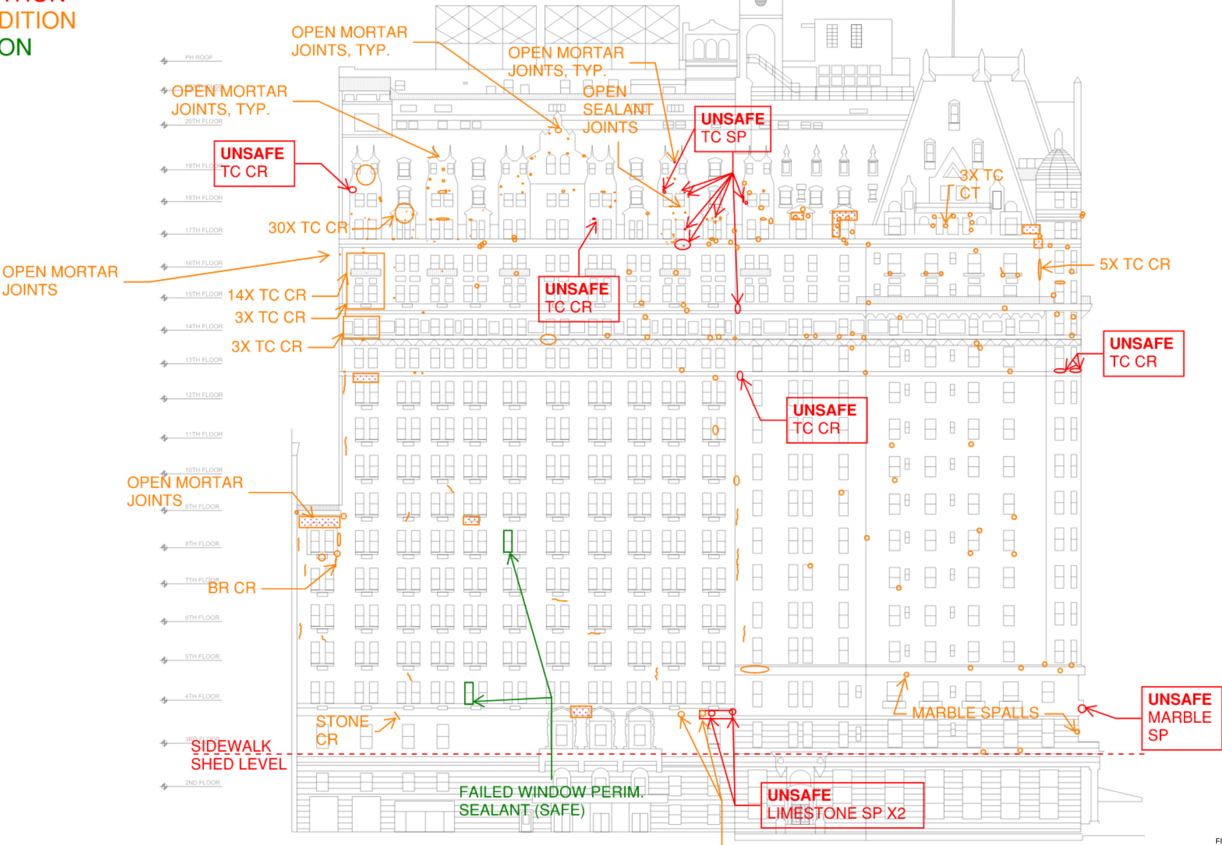
SOUTH ELEVATION - WEST 58TH STREET
